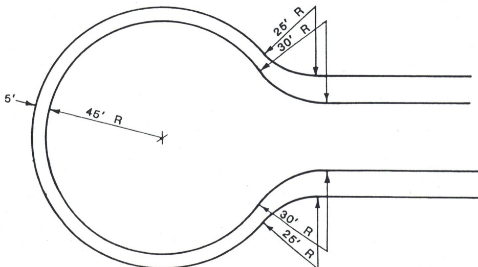
TYPICAL CUL-DE-SAC
