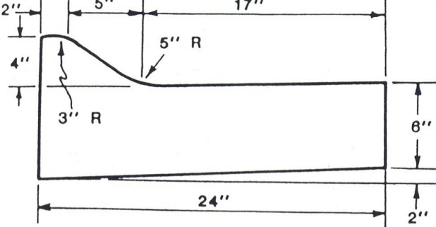
ROLLED CURB
