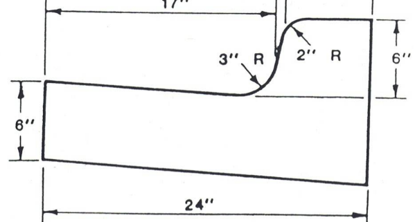
VERTICAL CURB
